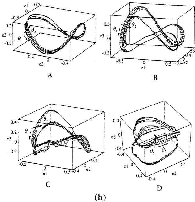
Figure 4: (a) The four objects used in the experiments. (b) The parametric hypersurfaces in object eigenspace computed for the four objects shown in (a). For display, only the three most important dimensions of each eigenspace are shown. The hypersurfaces are reduced to surfaces in three-dimensional space.
